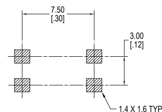
PC Layout
