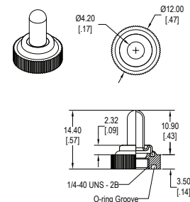
E - Sealed Boot Knurled Nut
