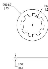
Lock Washer
